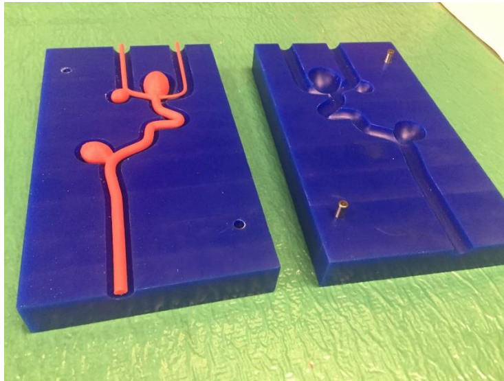
Figure 1: 3D printer inner core and CNC'ed outer core
